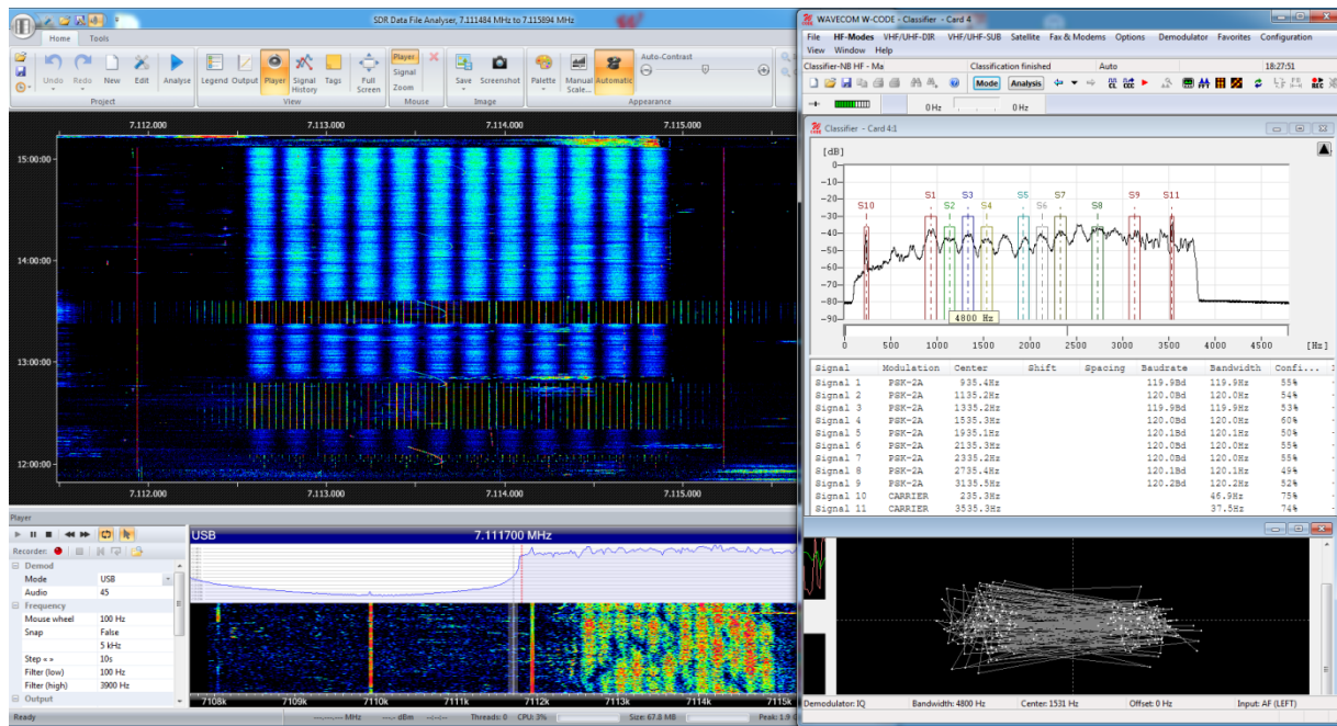
Figure 16: Here the OFDM-12 data signal around 7113,7 kHz (left, in the window of SDR-COM2) has been classified by Wavcom's W-Code (right). Due to some interference, the classifier got eleven channels of the signal. Below at the right you see the phase plane of the PSK-2A signal. This example shows also, that under interference you cannot rely completely just on automatic classification.
