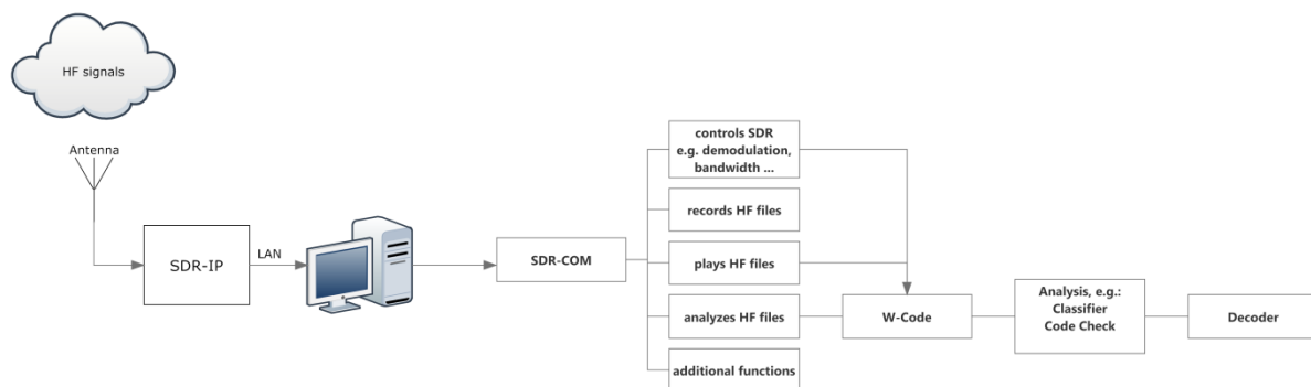
Figure 1: Example for a high-end receiving post. It consists of an SDR-IP from RFSpace 4 as receiver, locked to a GPS-driven frequency standard. The SDR is controlled by software SDR-COM2, and classification plus decoding of data transmission is done by software decoder W-Code of Wavecom 5 .
