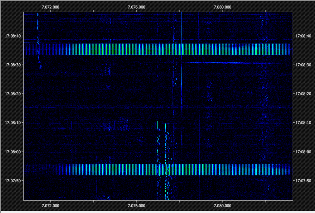
Figure 13: The two blocks of carriers are 3,75 seconds long and consist of carriers with a distance of 66,67 Hz.
